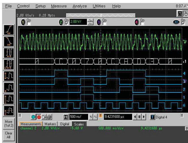
Figure 7. Digital signals can be grouped together by bus and viewed as hex value at every transition.
