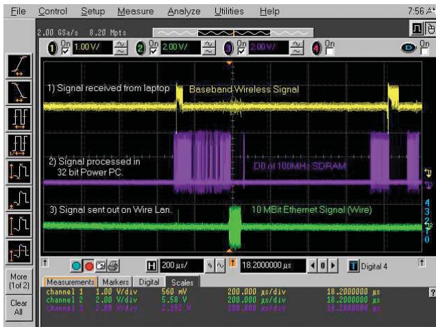
Figure 8. With an MSO, you can view a mix of signals. MegaZoom Deep memory lets you capture slow signals and then zoom in on the details fast without having to trigger twice.
