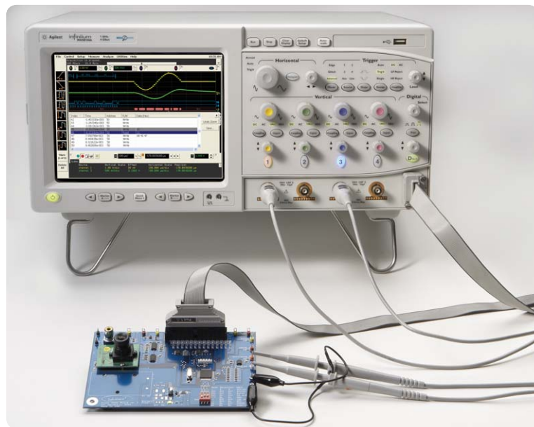
Figure 3. Using an Infiniium MSO8104A to probe the analog and digital signals of a wireless LAN access point.
