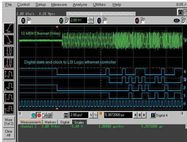
Figure 5. Use the MSO's 16 digital channels for triggering. The MSO is set to trigger on the 1010 pattern for a duration of 5 microseconds. With an ordinary four-channel DSO, the four channels would be used just to generate a trigger and there would be no channels left for debugging.
