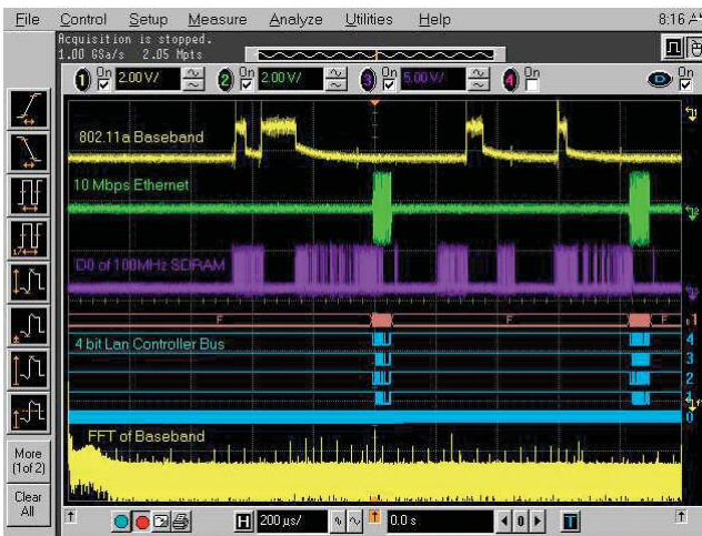
Figure 4. An MSO allows you to time correlate analog, digital, and spectral information all in one instrument.
